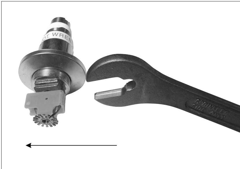
Fig. 12 - Model F3 or Model F3R Wrench
